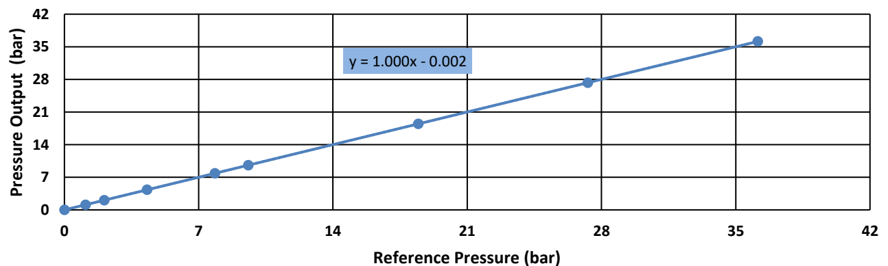
Pressure Output vs Reference Pressure
