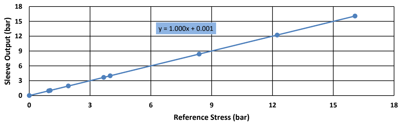
Sleeve Output vs Reference Stress
